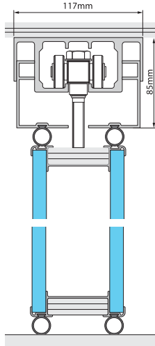
Top Hanging Vertical Cross Section
