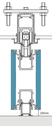
Type 110 Single Point Track
