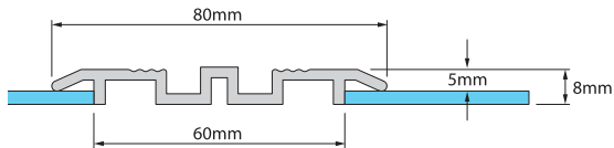
Low Profile Floor Track
