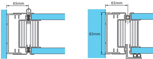
Low Profile Floor Track
