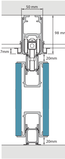
Type 85 Single Point Track
