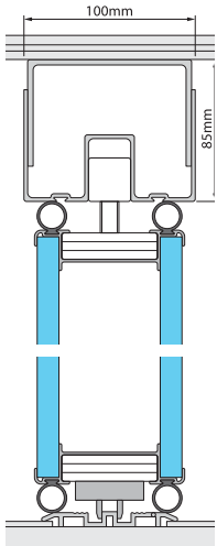
Floor Mounted Vertical Cross Section
