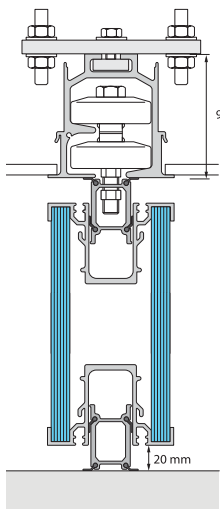
Type 100 Twin Point Track
