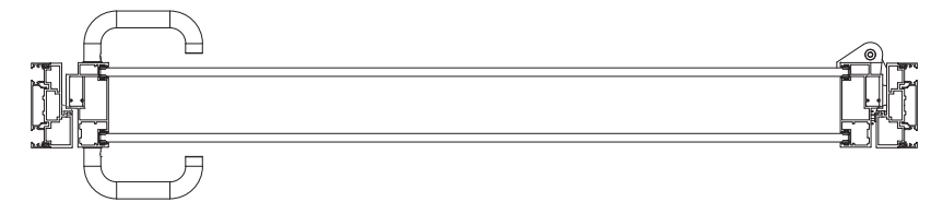
IN WALL STILE DOOR
